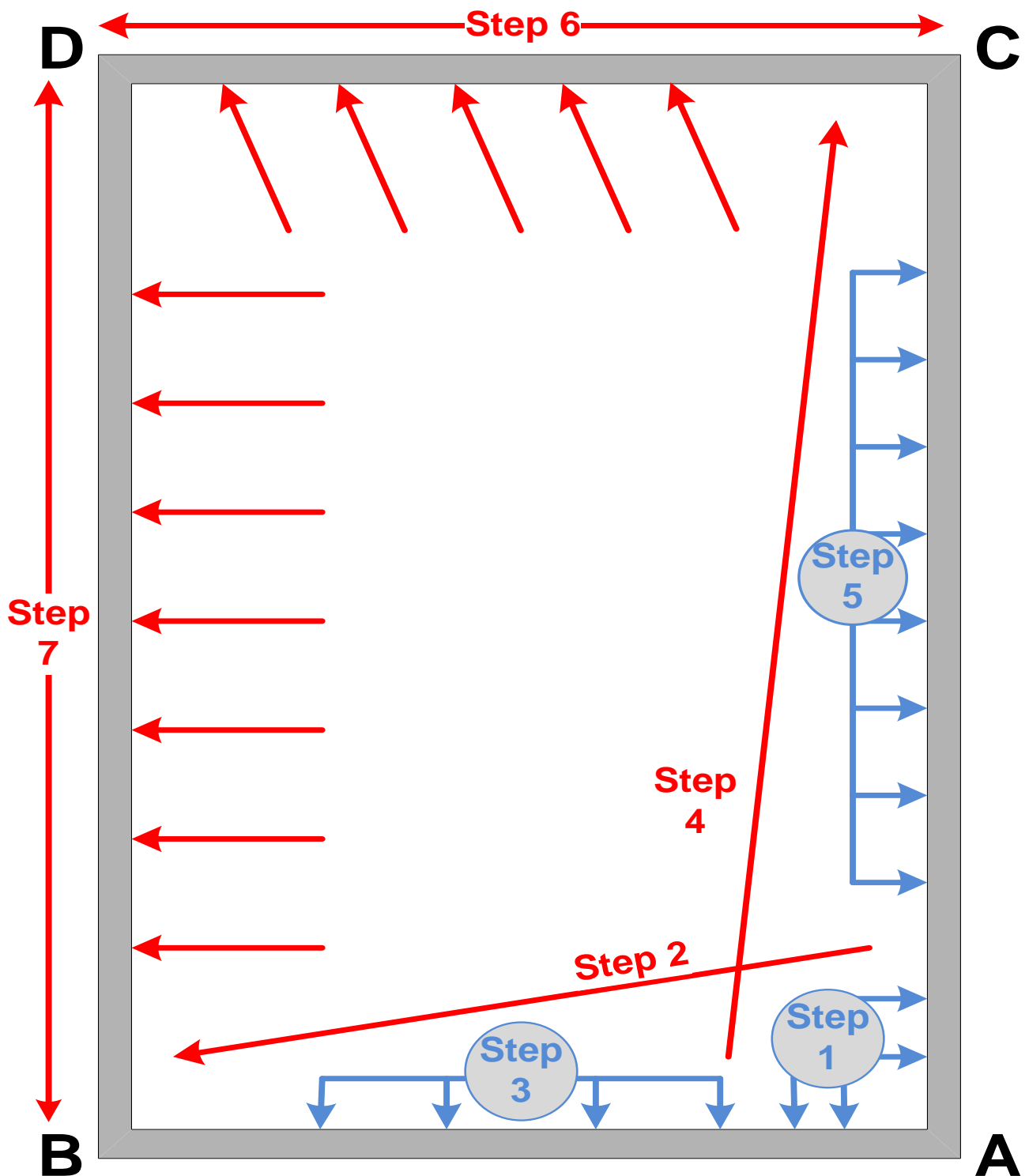
Figure 3: Stretch Diagram for Tufted Carpet In the absence of carpet manufacturer stretch recommendations, use this diagram.
